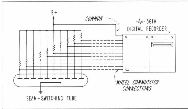
Fig. 5. Typical arrangement for feeding one column of printer from 10-element data device. Printer circuits are floating to permit operation from off-ground sources and have high input impedance so that source loading is small.
