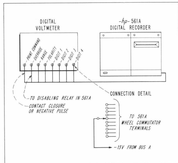
Fig. 4. Typical interconnection arrangement for using printer with digital voltmeter. Printer provides negative voltage source for feeding voltmeter contact closures.
